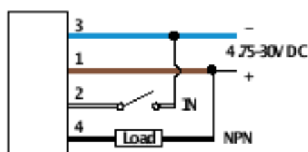
Figure 3. NPN
