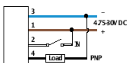
Figure 4. PNP
