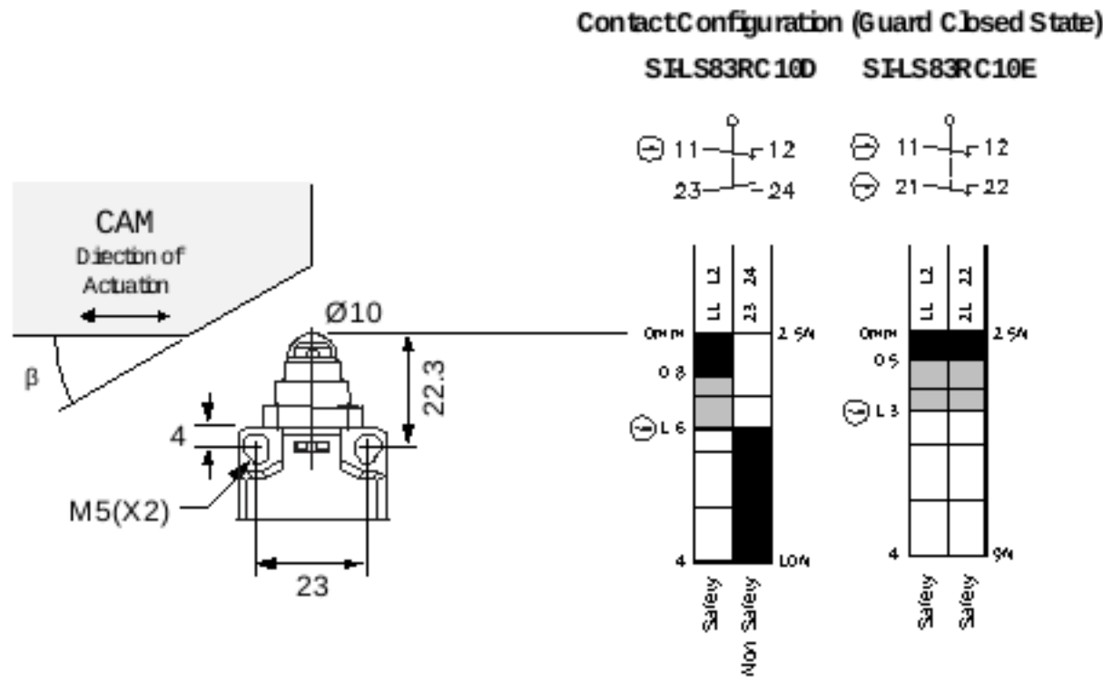
Figure 2. SI-L583RC10x Switching Diagrams
