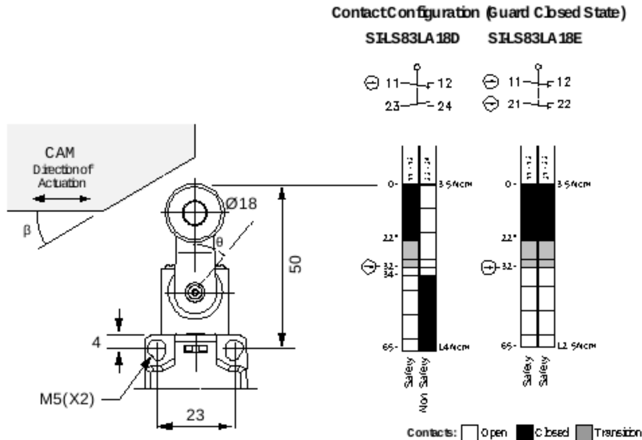
Figure 3. SIL583LA18x Switching Diagrams
