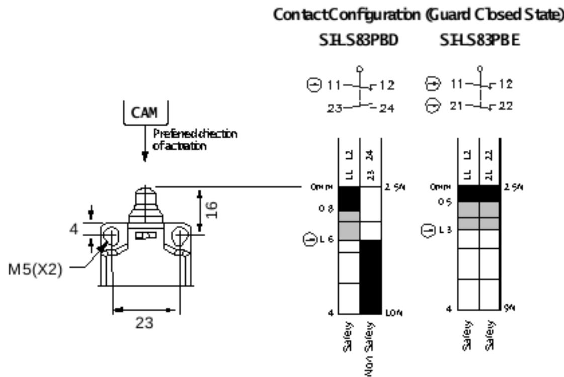
Figure 1. SLS83PBx Switching Diagrams
