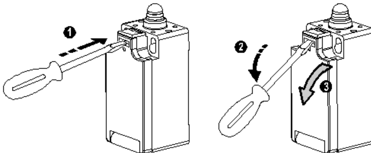
Figure 5. Accessing the Wiring Chamber
