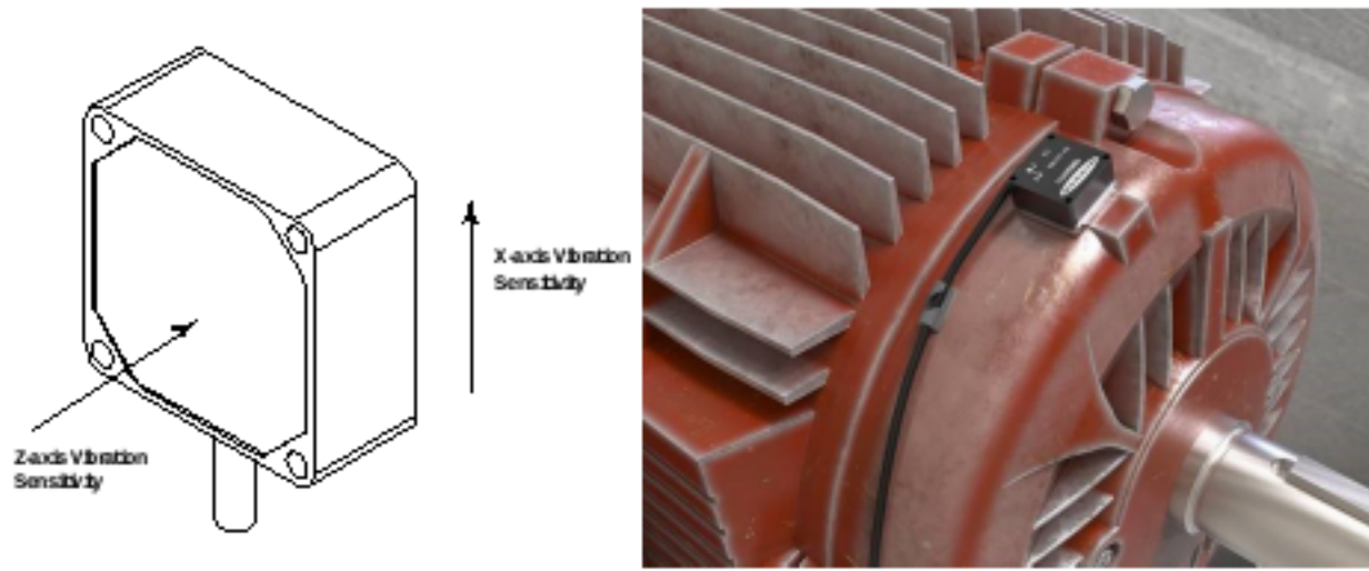
Figure 1. Installation direction
