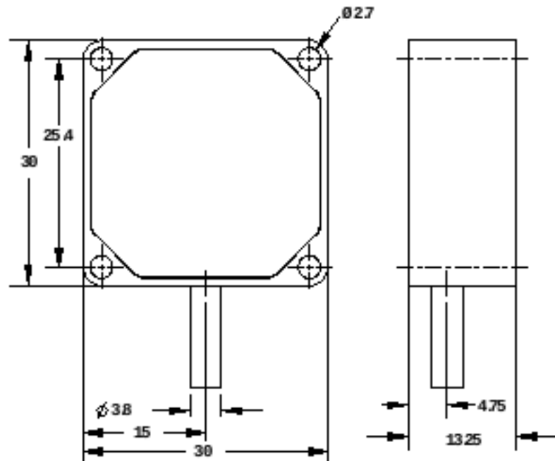
Figure 3. Aluminium model
