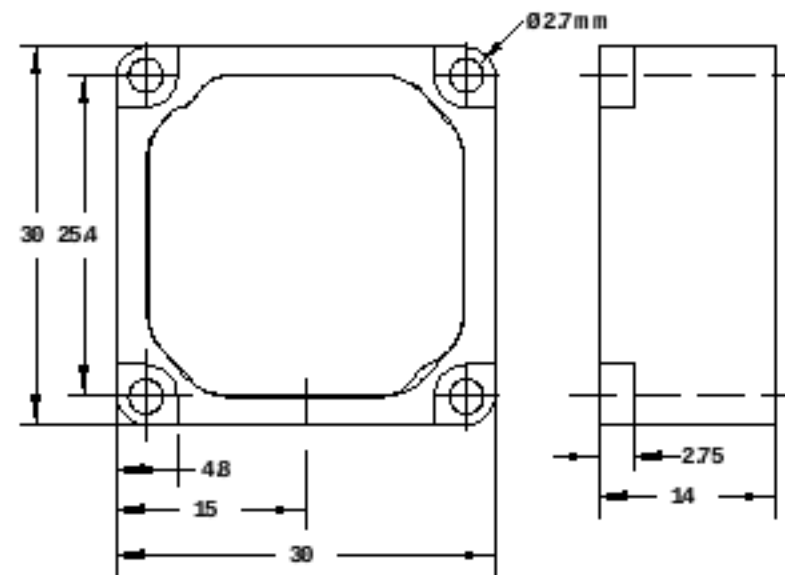
Figure 4. Stainless steel models
