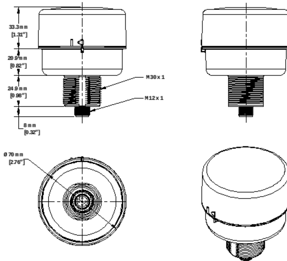
Figure 6. Dimensions for the R70SR
