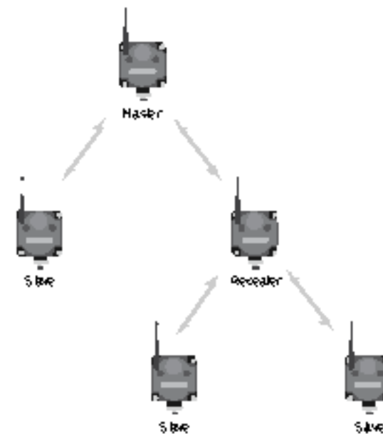
Figure 5. Tree network
