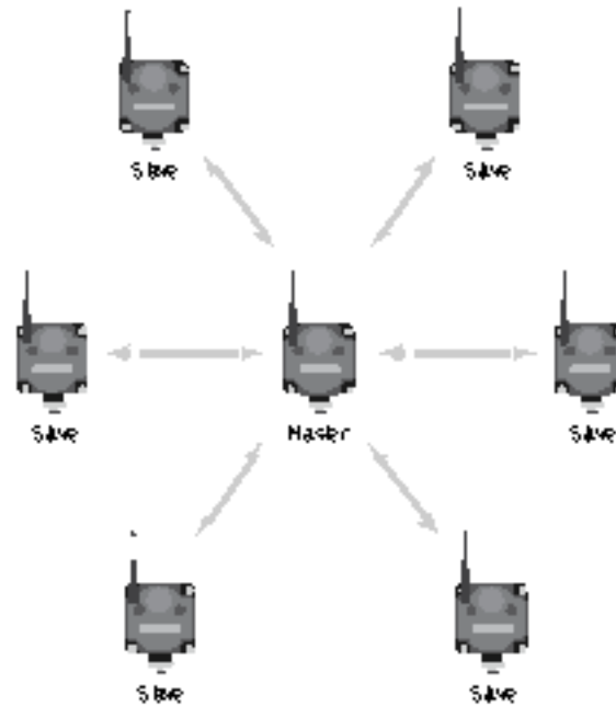
Figure 4. Star network
