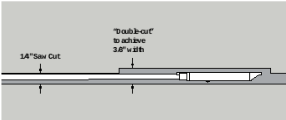
Figure 4. Sensor placed in saw cut in pavement
