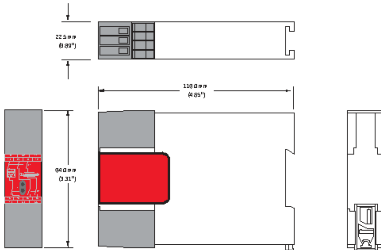
Figure 9. Interface module dimensions
