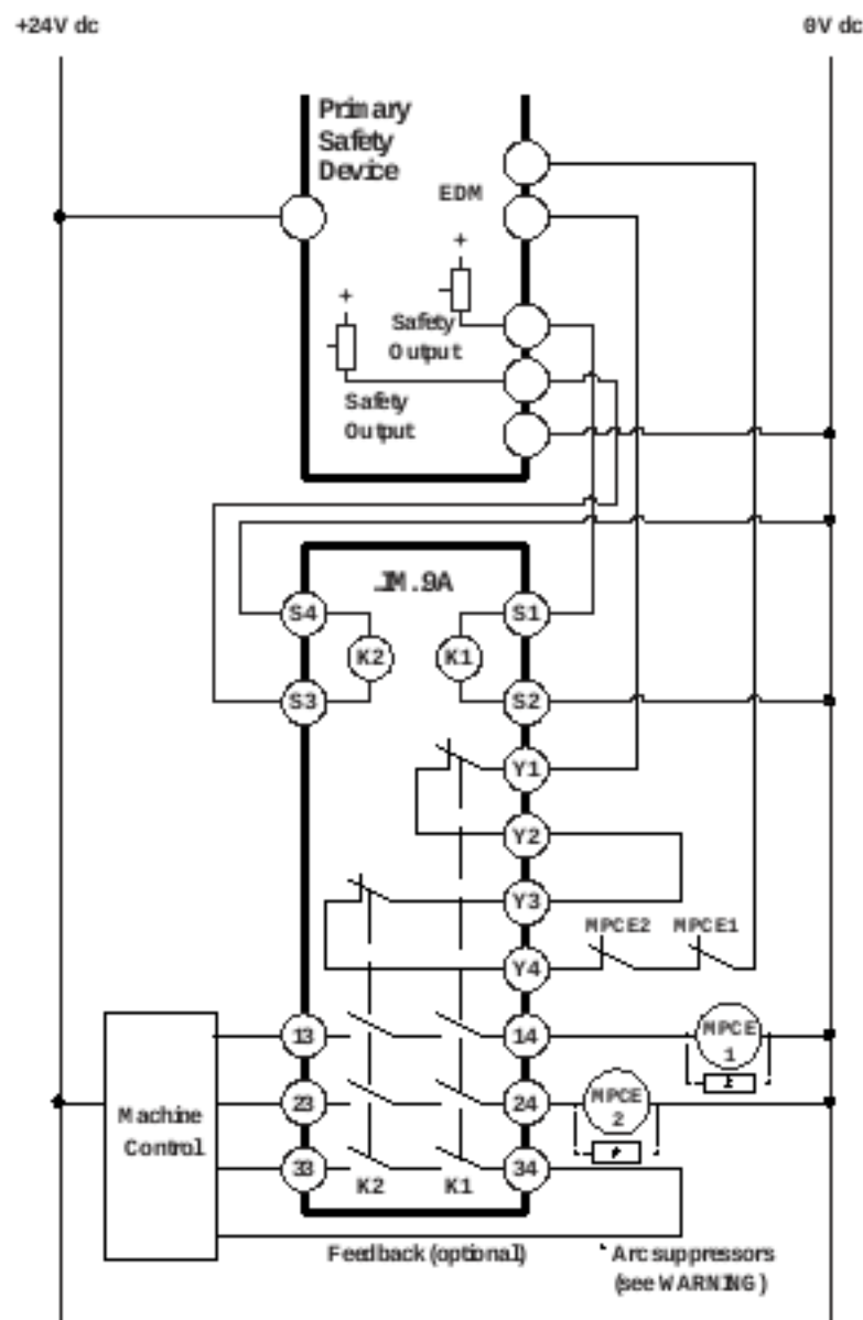
Figure 6. Generalized wiring to a 2-channel primary safety device with two current-sourcing safety outputs and one monitoring input.
