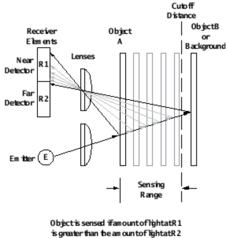
Figure 1. Fixed-Field Concept
