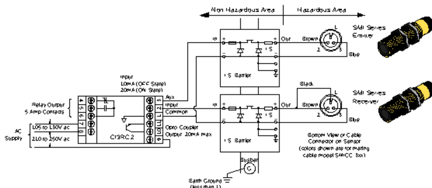
Figure 3. Hookup Using Two Single-Channel Barriers
