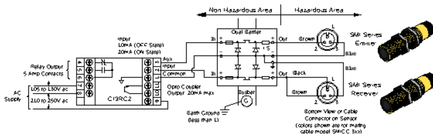
Figure 4. Hookup Using One Dual-Channel Barrier
