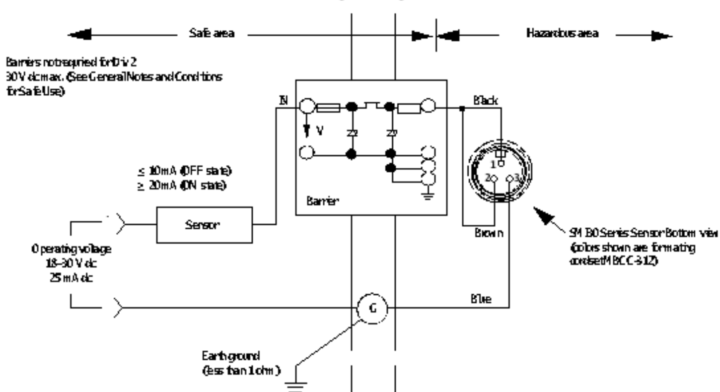
Figure 2. Wiring for 2-Wire Connections
