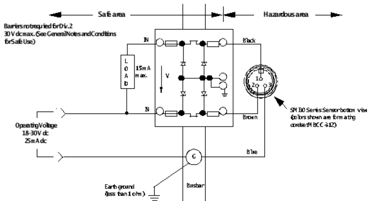
Figure 1. Wiring for 3-Wire Connections
