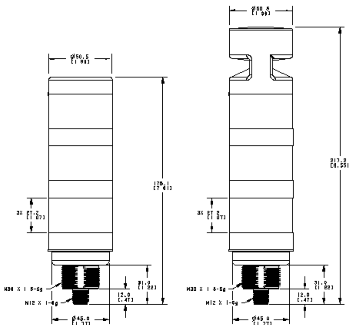
Standard Models
