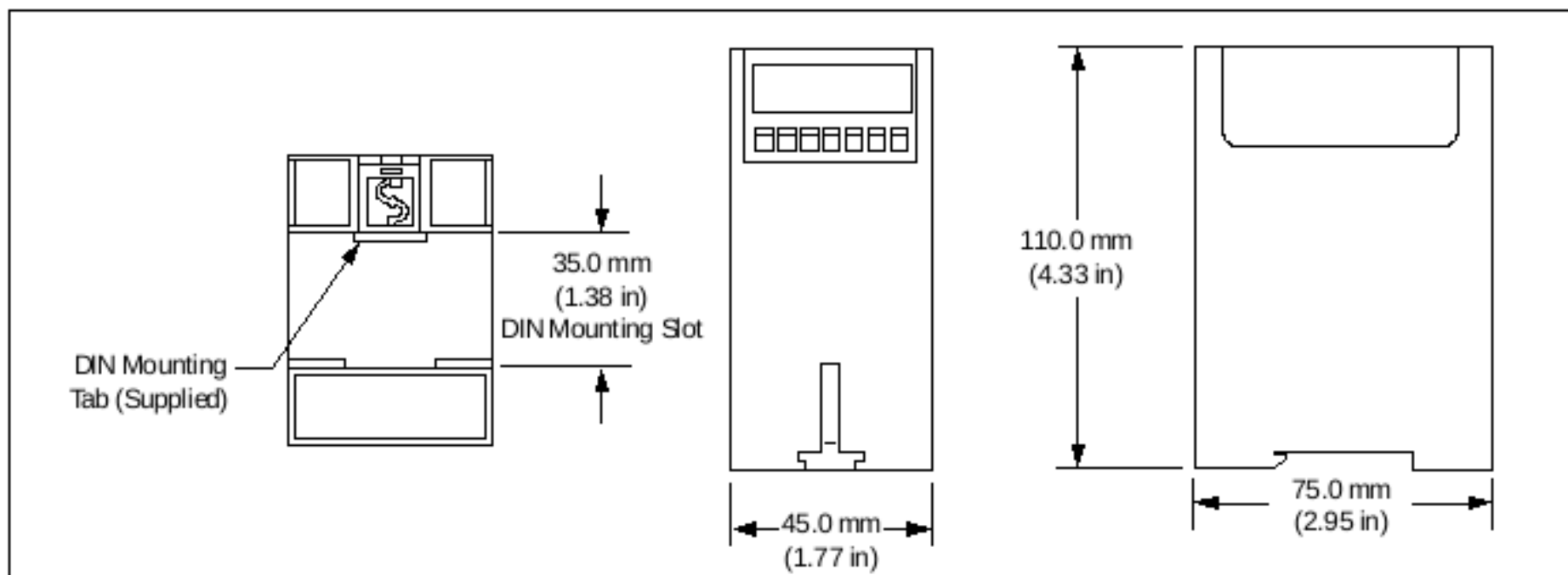
Figure 4. E-Stop Enclosure Dimensions
