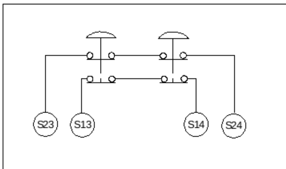
Figure 3. Series Connection of Multiple Emergency Stop Switches
