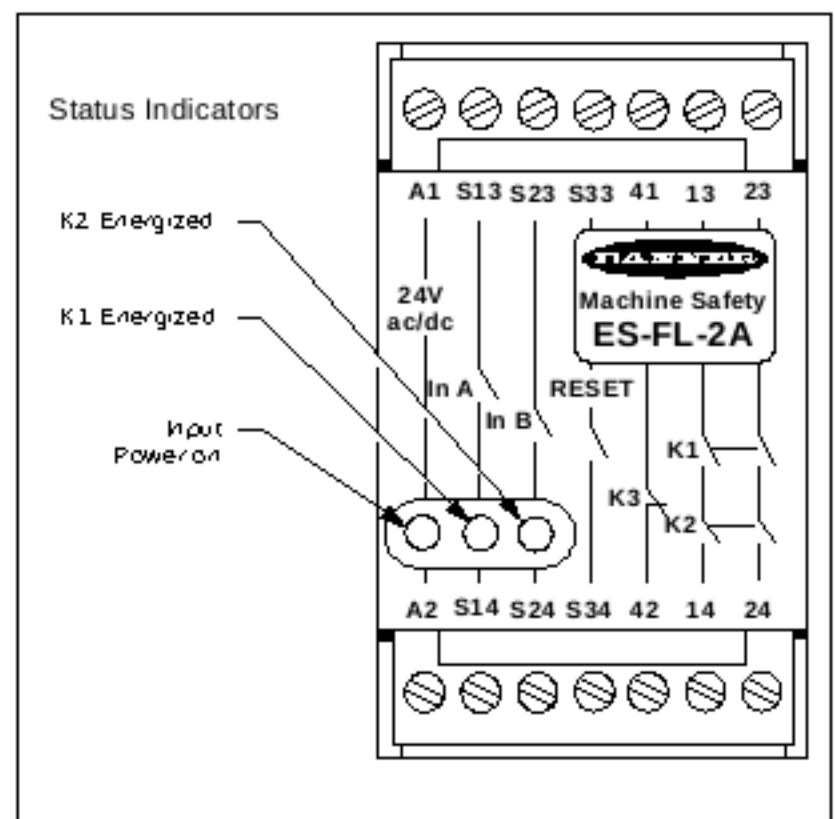
Figure 1. ES-FL-2A Status Indicators
