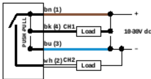
Figure 1. Channel 1 = IO-Link, Channel 2 = PNP Output
