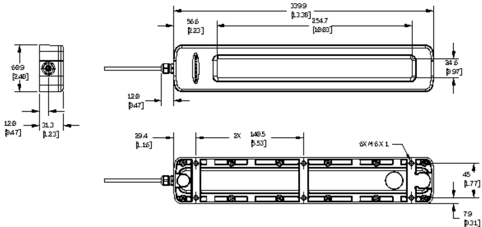
Figure 1. WLH60 (340 mm) Base Mount Side Exit Model
