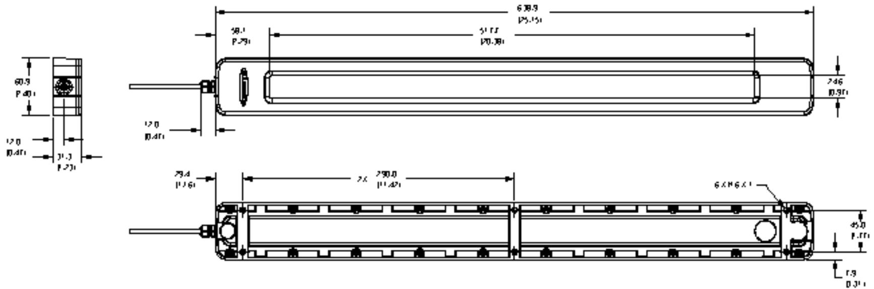
Figure 2. WLH60 (640 mm) Base Mount Side Exit Model
