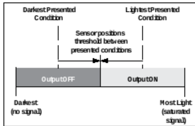
Figure 4. Dynamic TEACH (Light Operate shown)
