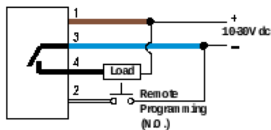
NPN (Sinking) Outputs
