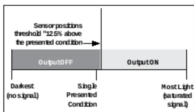
Figure 6. Dark Set (Light Operate shown)
