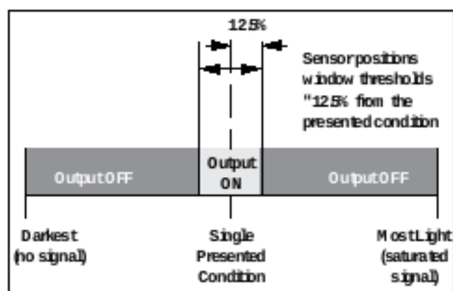
Figure 7. Window Set (Light Operate shown)
