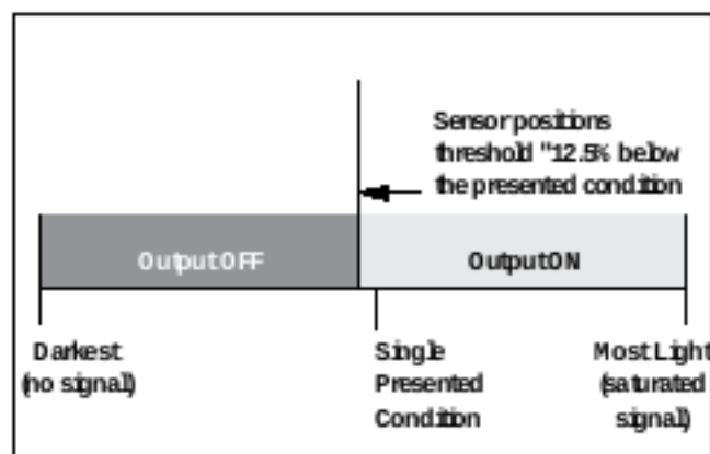
Figure 5. Light Set (Light Operate shown)
