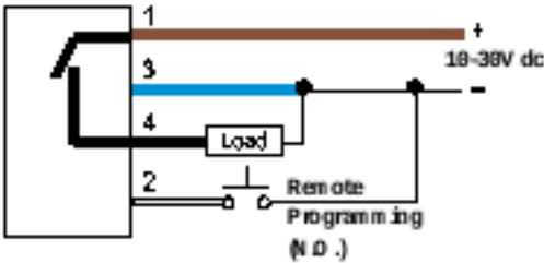
PNP (Sourcing) Outputs
