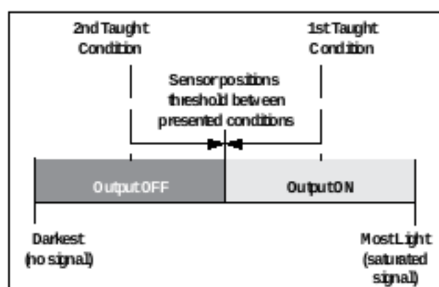
Figure 3. Static TEACH (Light Operate shown)
