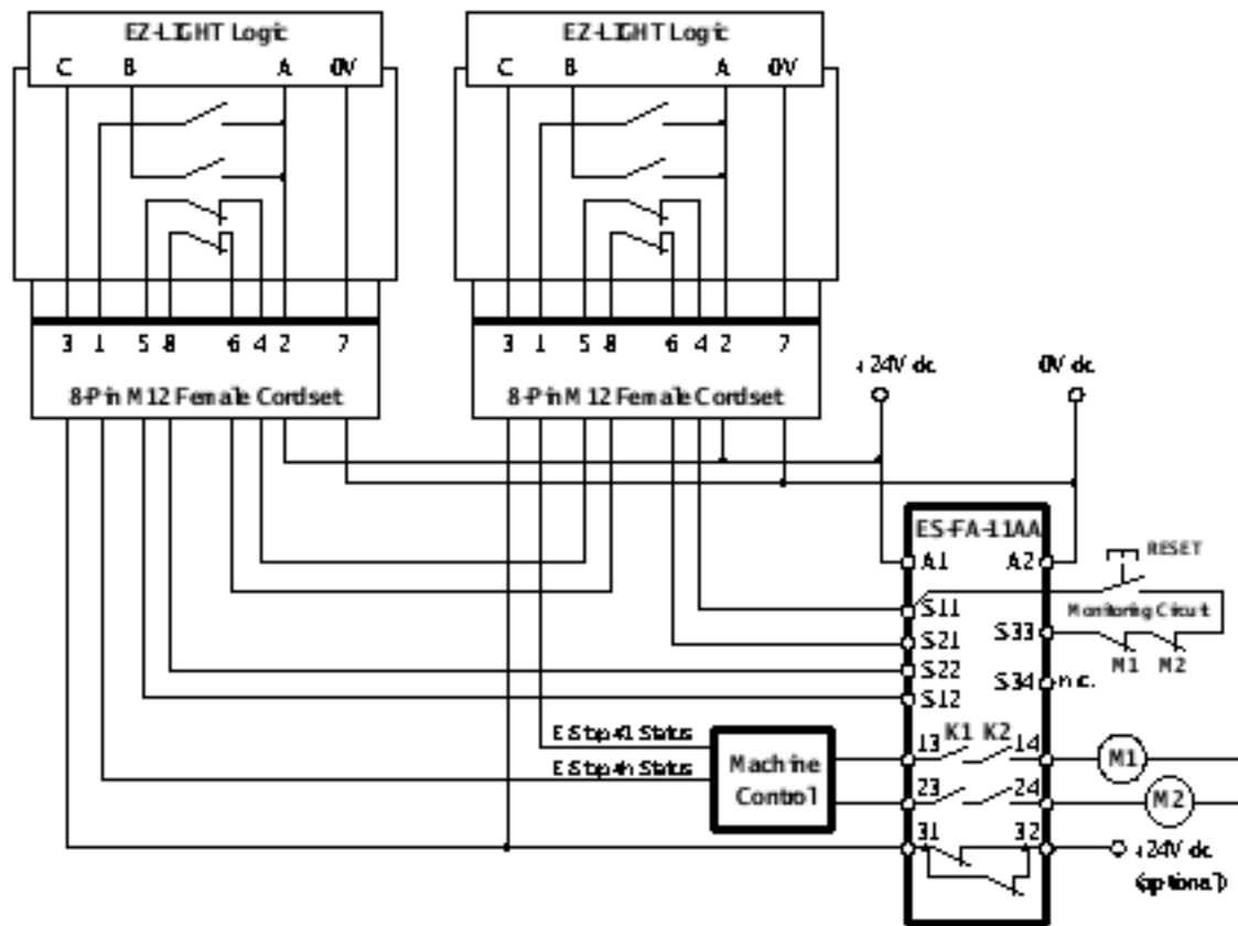
Figure 1. Illuminated Models—Example Hookup
