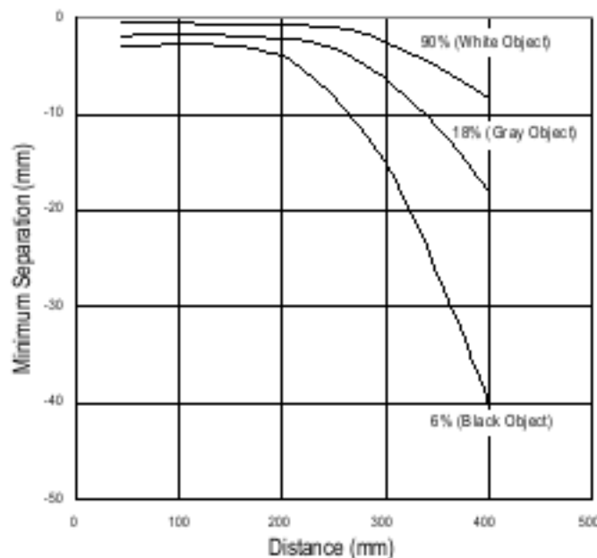
Minimum separation distance* between object and background: foreground suppression mode
