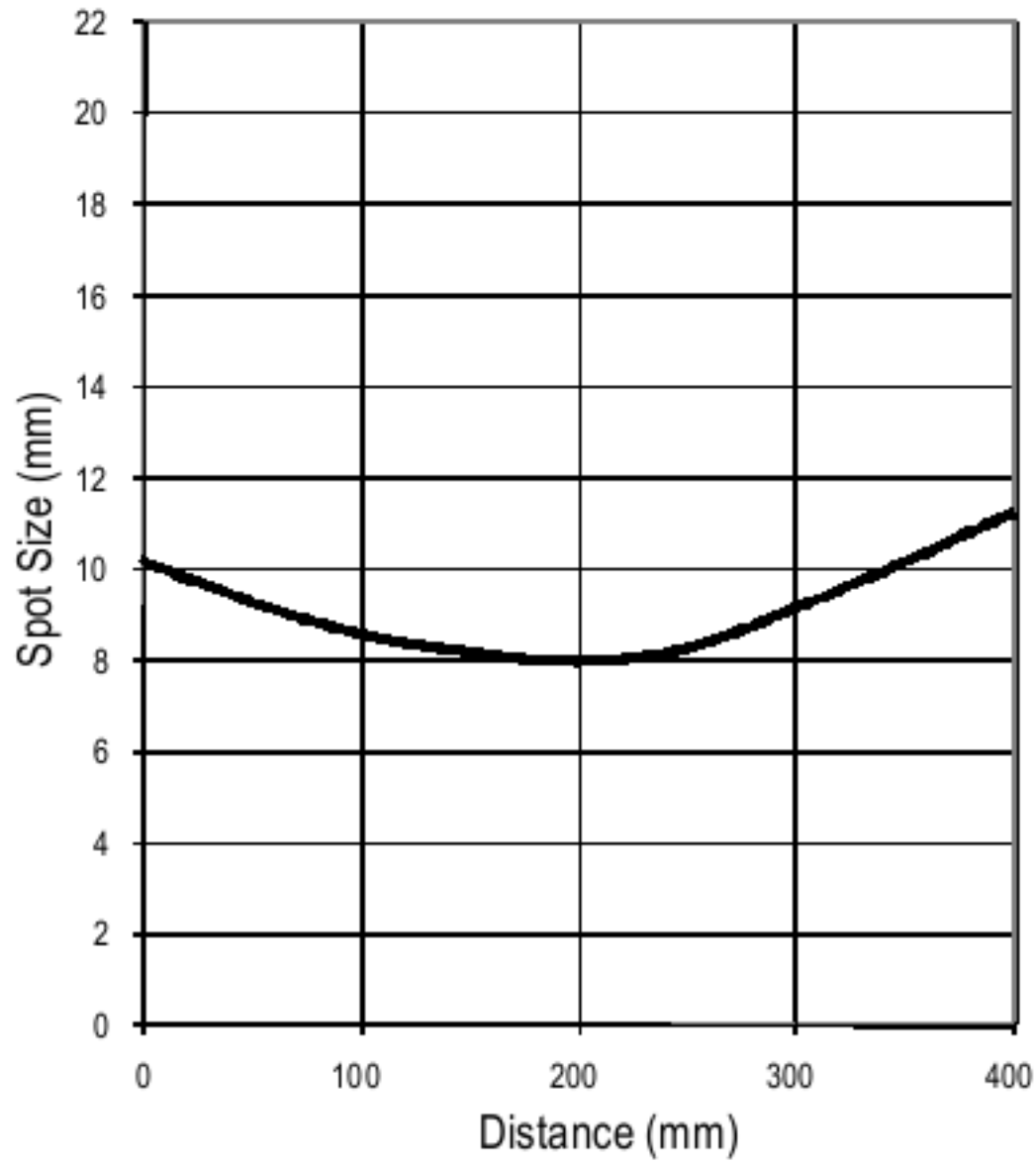
Typical emitter spot diameter vs. distance
