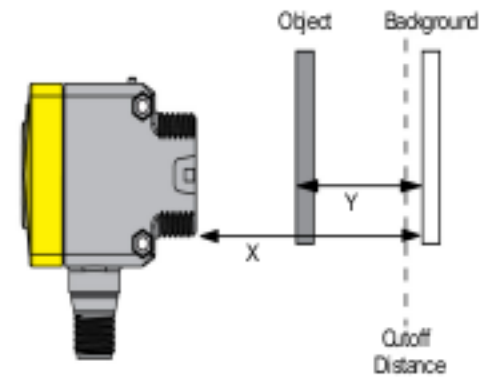
Set cutoff distance in front of the fixed background
