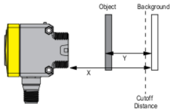
Minimum separation distance* between object and background: foreground suppression mode
