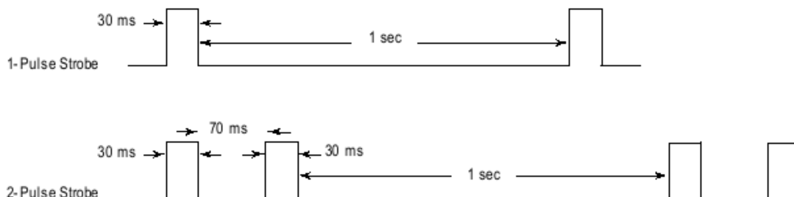
Timing diagram for 1 pulse or 2 pulses
