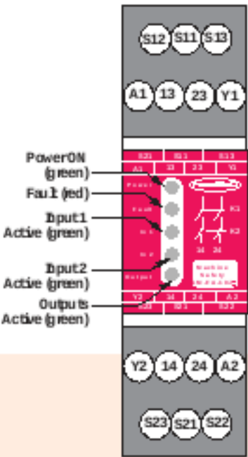
GM-FA-10J Features and Terminal Locations
