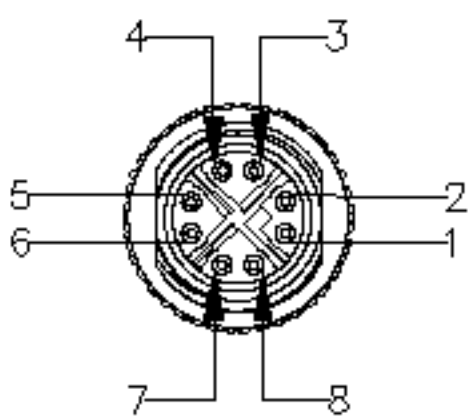
PIN OUT
