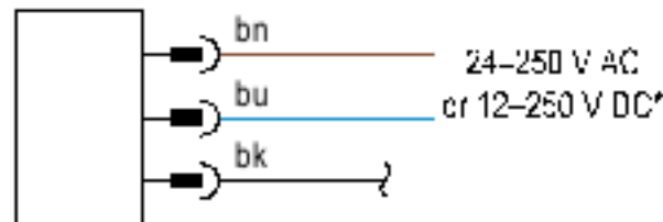
Q453EQ Emitters with Quick-Disconnect 3-Pin 7/8 in-16UNF
