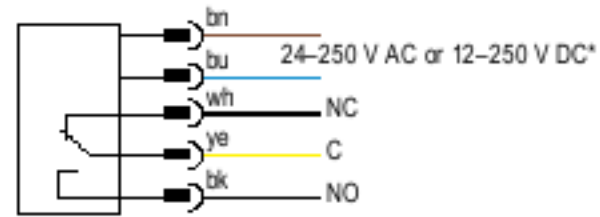
Q45VR3 Sensors with Quick-Disconnect 5-Pin 7/8 in-16UNF (model suffix Q)
