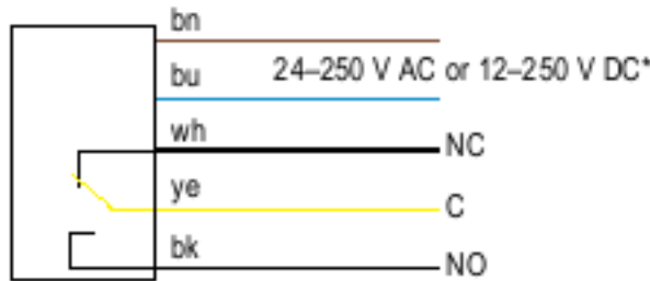
Q45VR3 Sensors with Attached Cable
