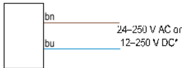
Q453E Emitters with Attached Cable
