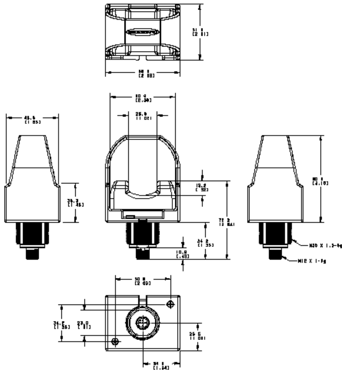
OTB with M12 Quick-Disconnect
