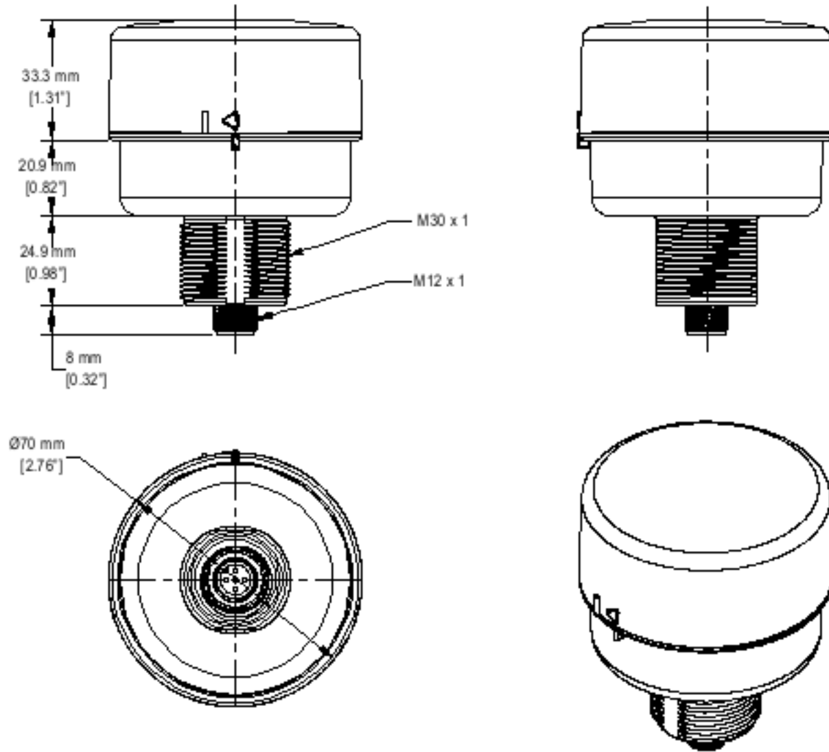
Dimensions for the R70SR
