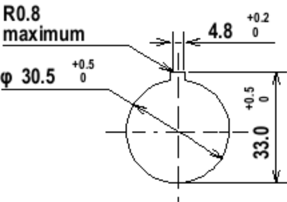
Notch dimensions
