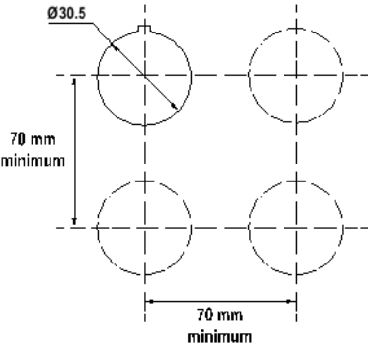
Notch dimensions
