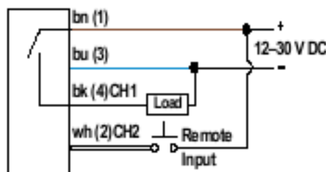
Channel 1 as PNP Output, Channel 2 as Trigger Input
