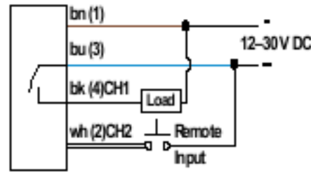
Channel 1 as NPN Output, Channel 2 as Trigger Input
