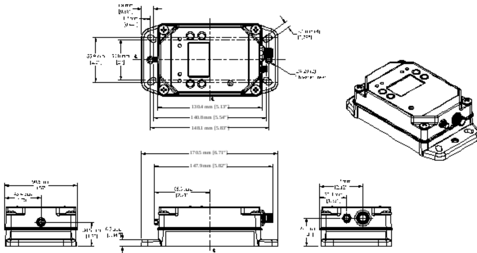
DXM1200 dimensions
