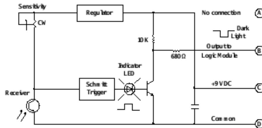
Figure 1. Functional schematic
