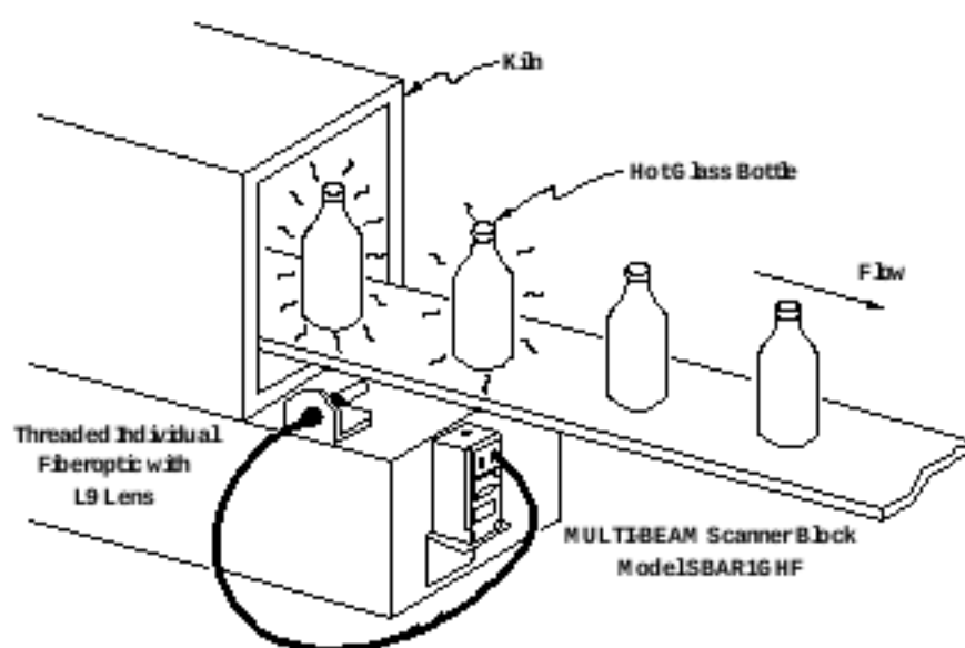
Figure 2. Direct Sensing of Radiant Infrared Energy
