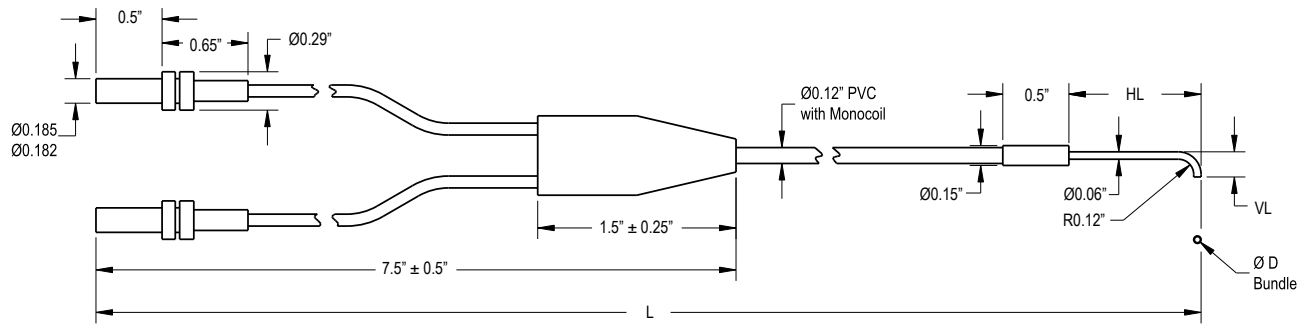
BMAP.753P Series Fibers
