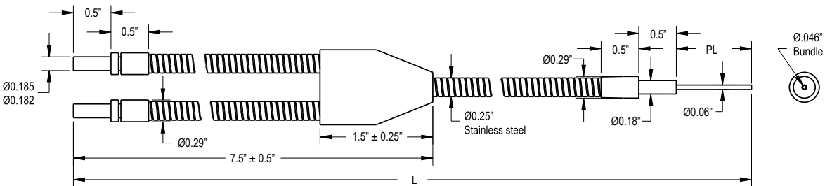
BM.75xS Series SS Terminated Glass Fibers
