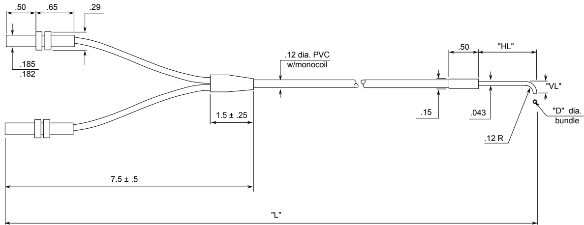
BMAP.442P Series Fibers
