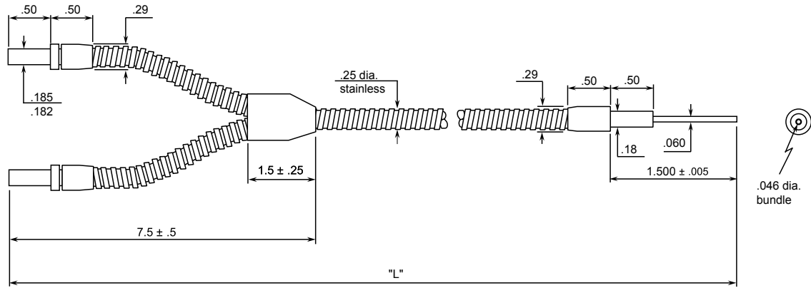
BM.752SMCTPL Series Fiberoptic Assembly
