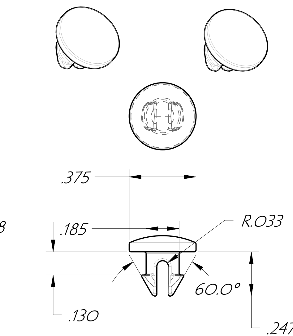
PLUG
