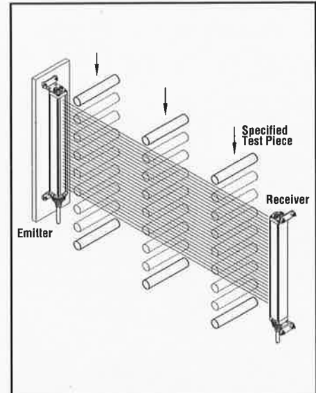
Figure 2. MINI-SCREEN System trip test
