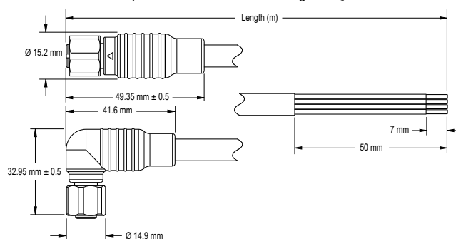
4-pin A-Code M12 Female Large Body
