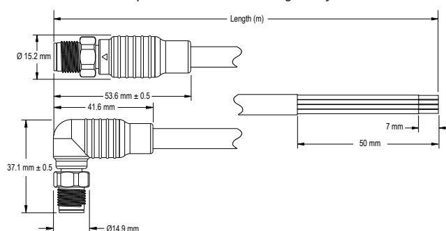
4-pin A-Code M12 Male Large Body
