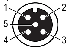
5-pin A-Code M12 Female
