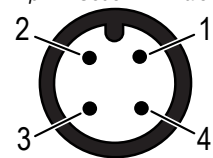
4-pin A-Code M12 Male
