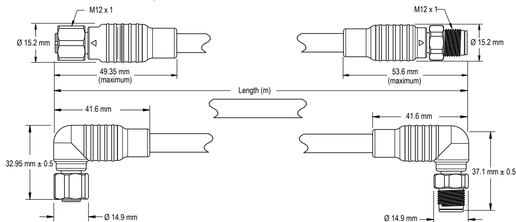
4-pin A-Code Double-Ended M12 Female to M12 Male
