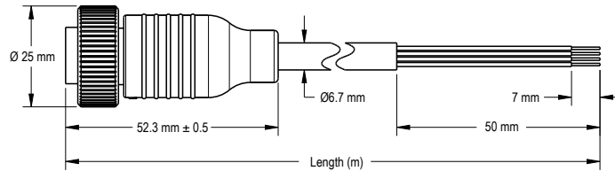
Single-Ended Mini Female
