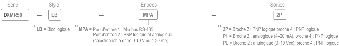
Ports DXMR50-LB-MPA
