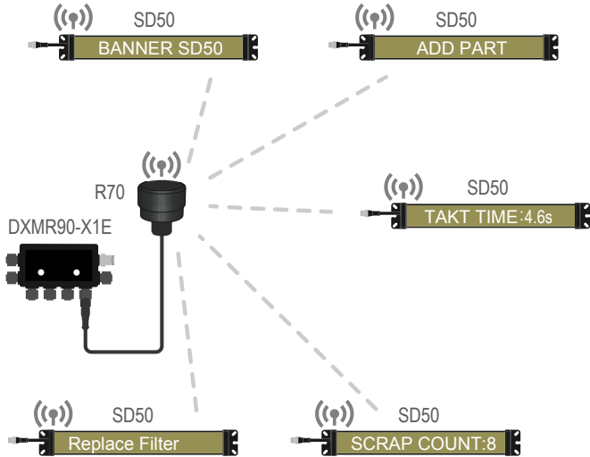
Example SD50 Wireless network layout (star topology)
