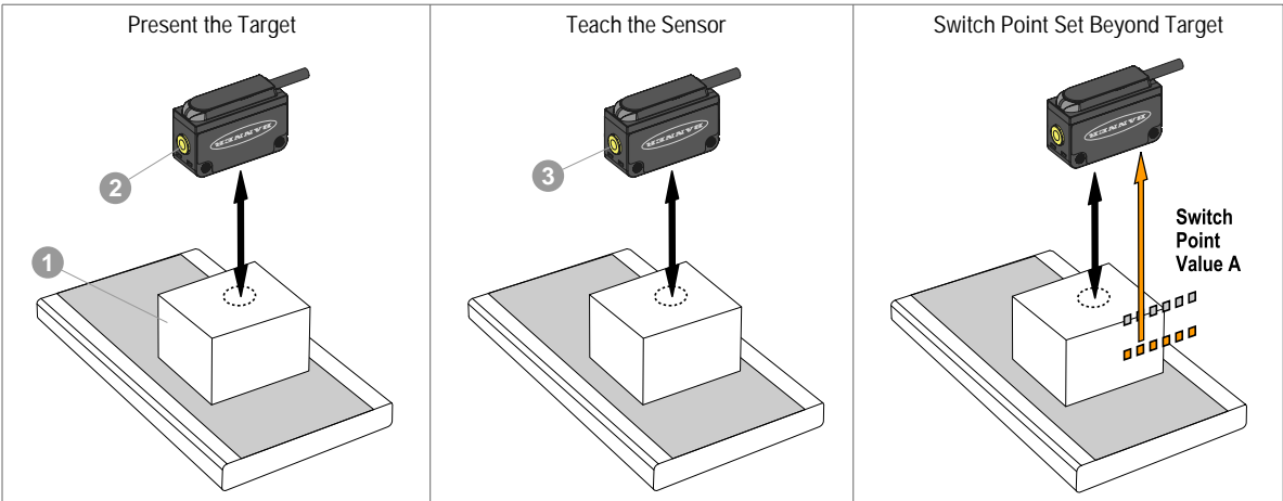
Figure 8. TEACH Process for One-Point Object SET
