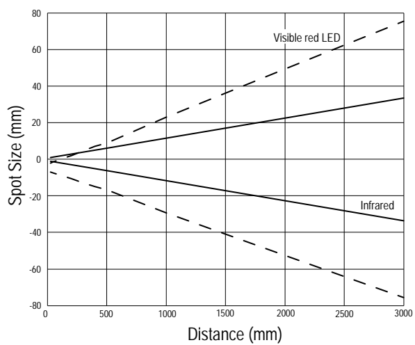
Figure 11. Spot Size
