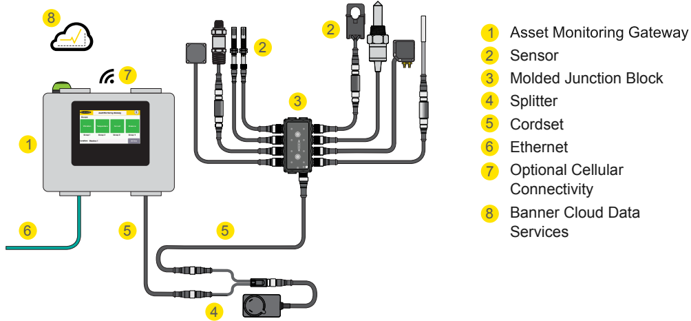
Connection example with limitless combinations of SNAP ID sensors and connectivity accessories
