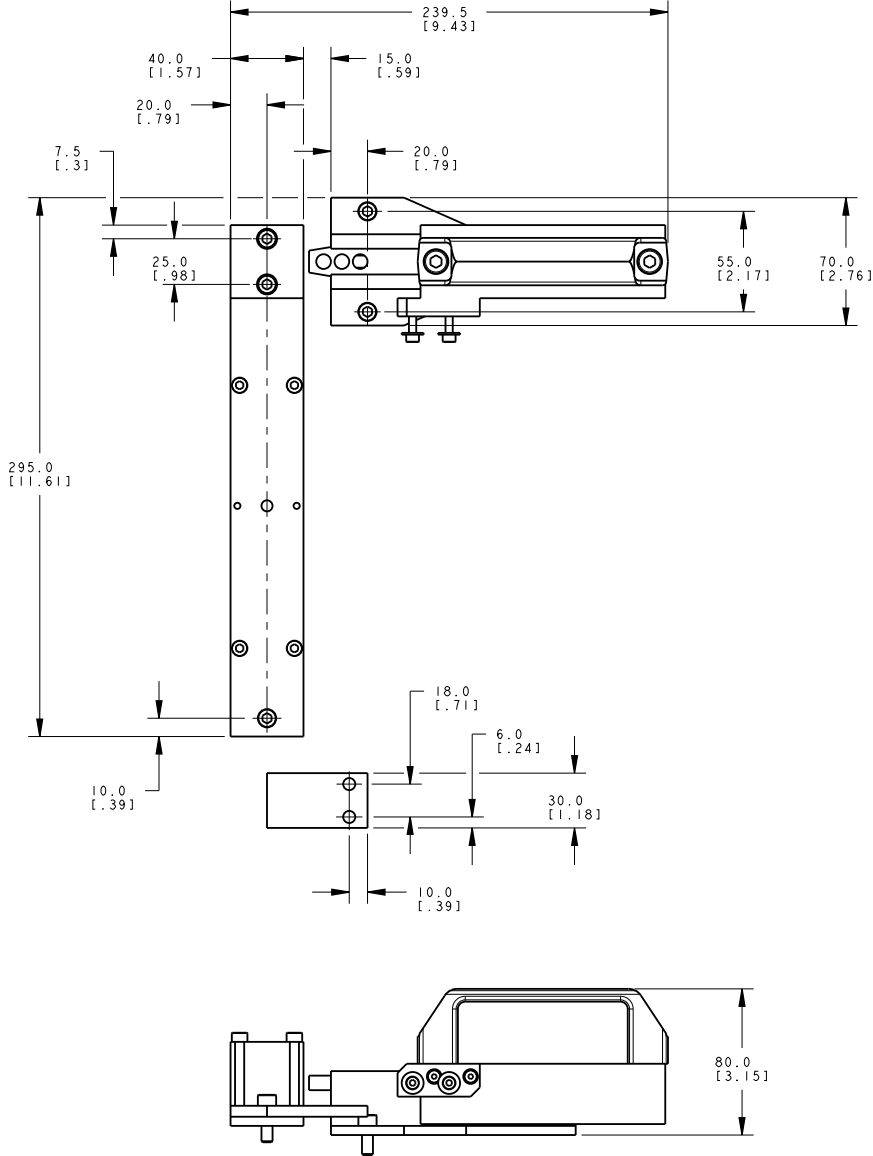
SI-QM-SSA-SH Right Hinge
