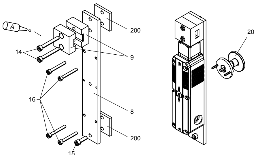
Base Plate Assembly of the SI-QM-SSA-SHER
