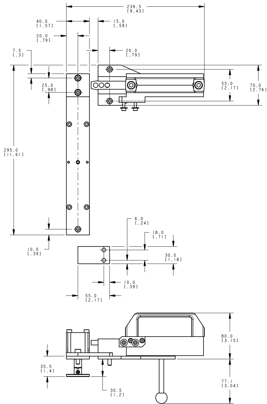
SI-QM-SSA-SHER Right Hinge
