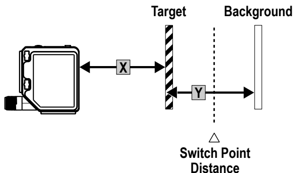
Figure 16. Minimum Object Separation Distance (90% to 6% reflectance) for the 3000 mm Models
