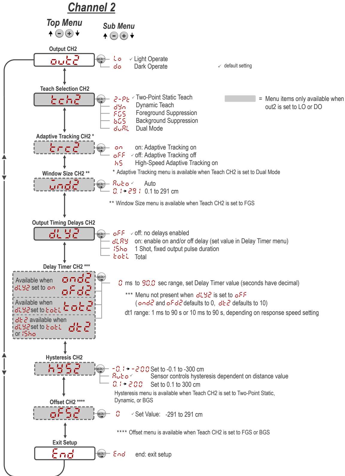
Figure 14. Sensor Menu Map—Channel 2
