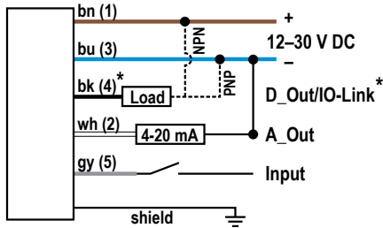
Figure 11. Wiring diagram for 4-20mA Analog
