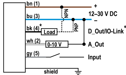
Figure 12. Wiring diagram for 0-10V Analog
