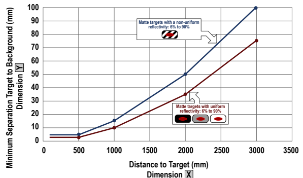
Figure 17. Discrete Minimum Object Separation (Uniform and Non-Uniform)
