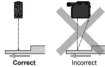
Figure 8. Orientation for a height difference
