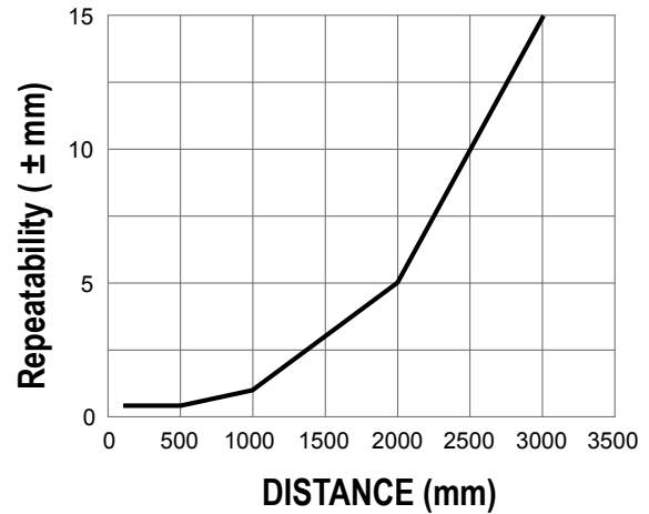
Figure 19. Repeatability (90% to 6% Reflectance)
