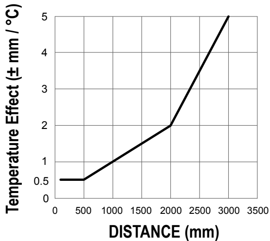
Figure 20. Temperature Effects (90% to 6% Reflectance)
