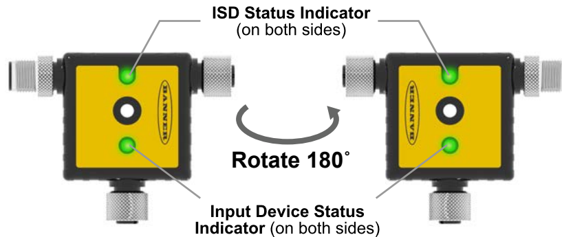
Figure 11. SSA-ISD Connect status indicators
