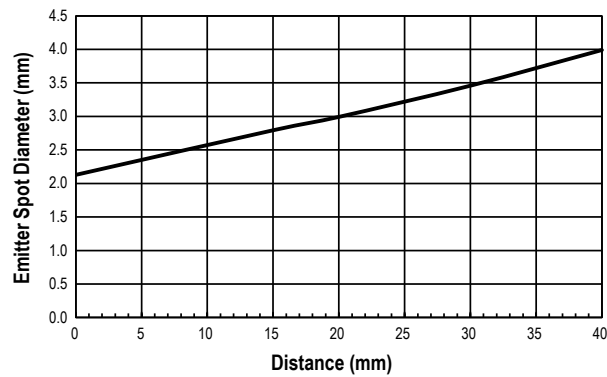
Figure 4. Typical Emitter Spot Diameter vs. Distance
