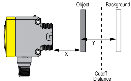
Minimum separation distance* between object and background: background suppression mode
