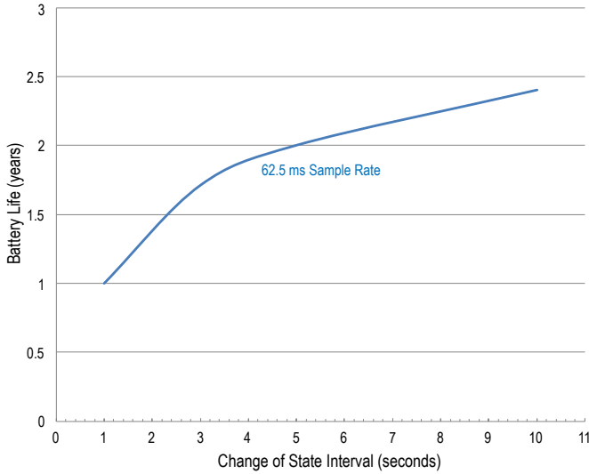
Battery Life for 900 MHz Radios
