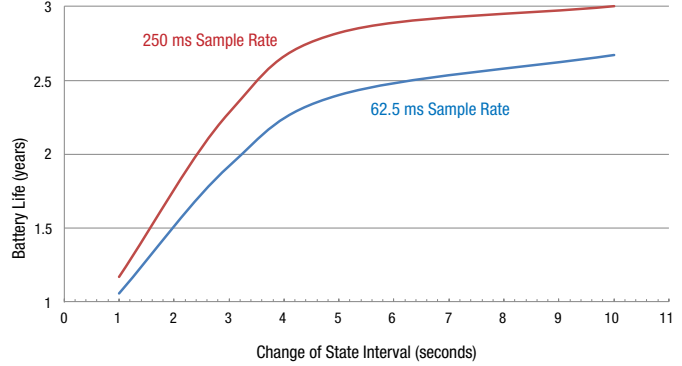
DX80N2Q45RD Battery Life
