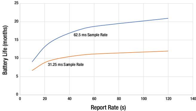
Battery Life for 900 MHz Radios
