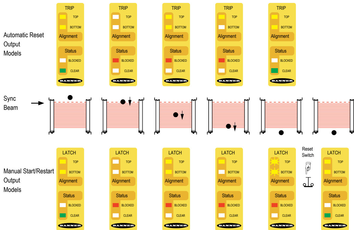
Figure 32. Status indicator behavior during the trip test
