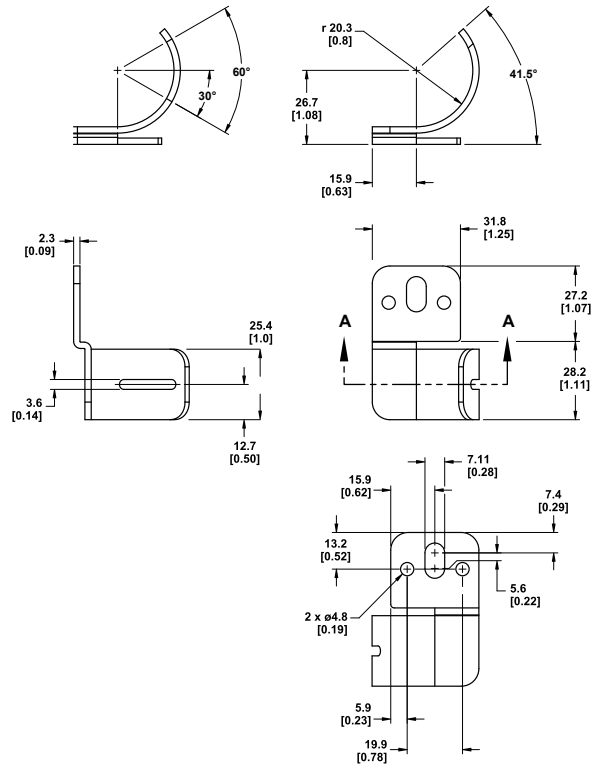
Figure 5. Mounts to a flat surface with the clamp piece
