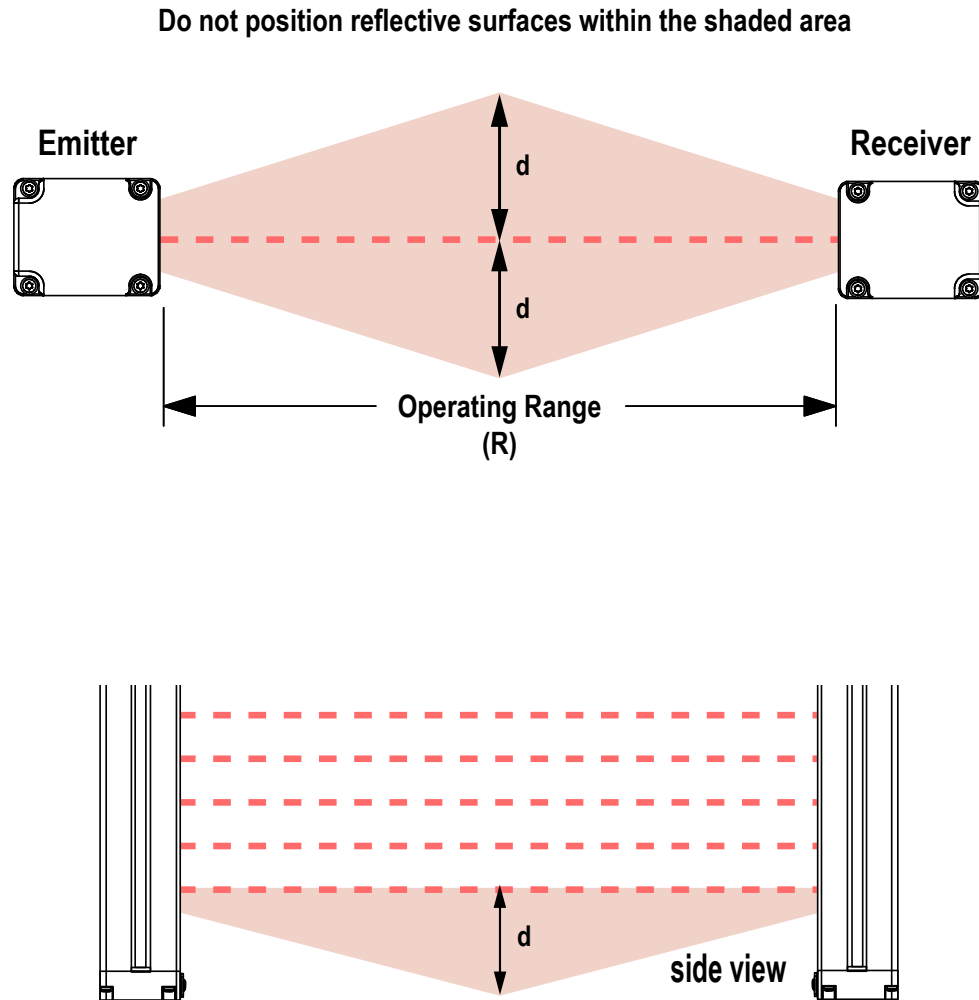
Figure 11. Adjacent Reflective Surfaces
