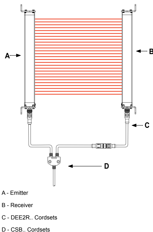
Figure 7. Splitter cordsets
