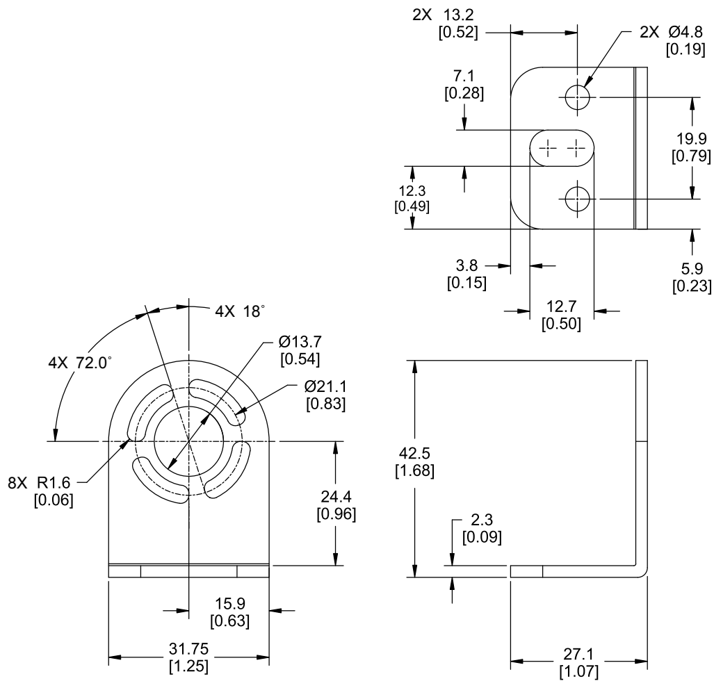
Figure 3. USMB-10 Bracket
