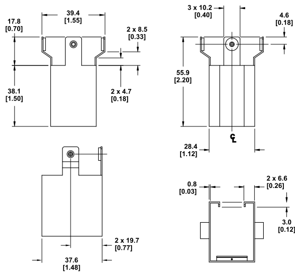
Figure 4. Clamp piece attaches to the EZ-SCREEN
