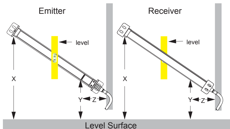
Figure 18. Angled or horizontal installations
