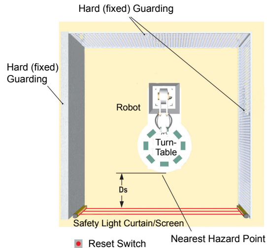
Figure 9. Safety distance (minimum distance) and hard (fixed) guard
