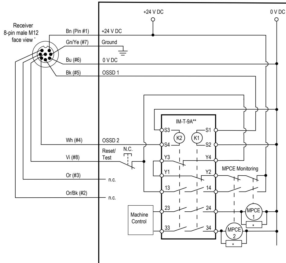
Figure 31. Generic Wiring — Interface Module (2-Channel EDM, Manual Reset)
