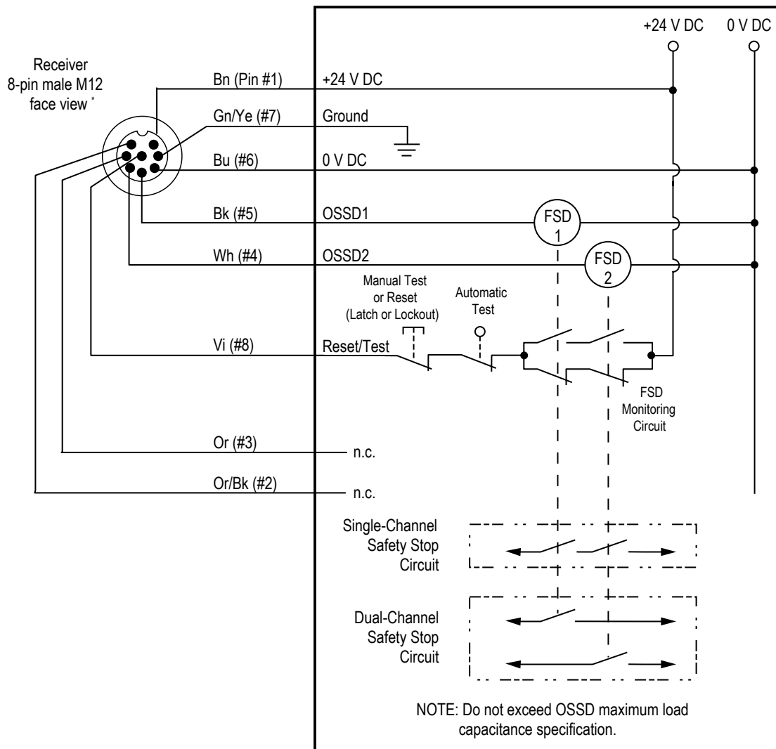
Figure 30. Generic Wiring to FSDs (manual reset)
