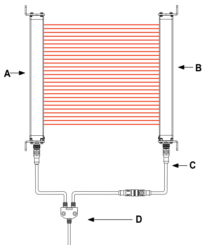
Figure 22. Splitter cordsets
