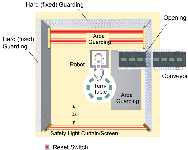
Figure 10. An example of supplemental safeguarding
