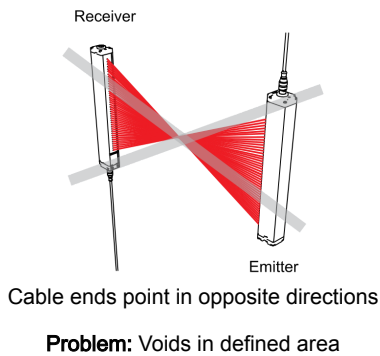
Figure 14. Examples of Incorrect Emitter/Receiver Orientation
