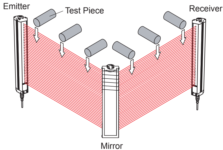
Figure 28. Trip Test with Corner Mirror
