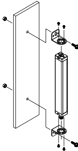
Figure 16. Emitter and receiver end-cap mounting brackets
