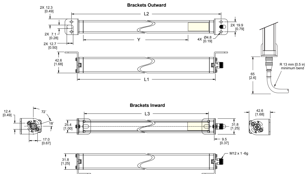
Figure 2. Dimensions
