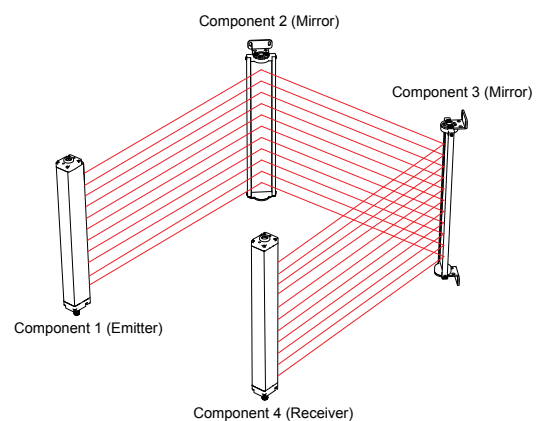
Figure 26. Corner Mirror Alignment
