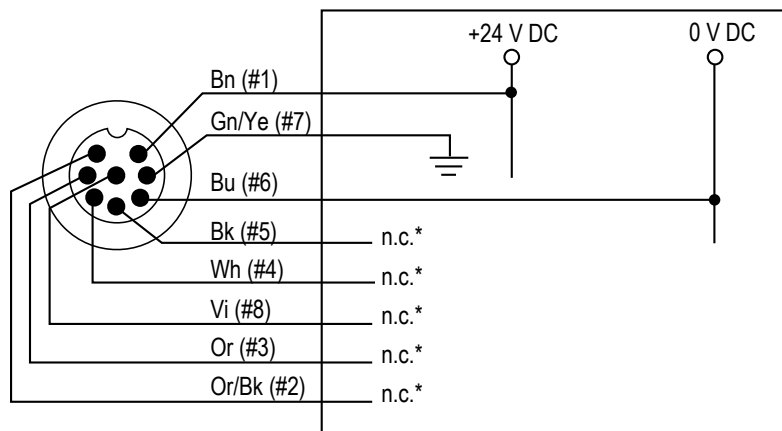
Figure 29. Emitter—Generic Wiring Diagram
