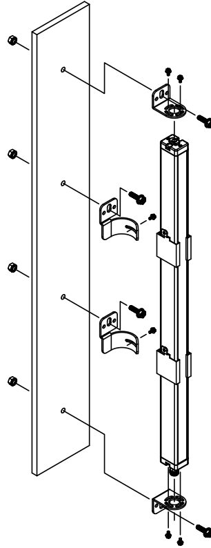
Figure 17. Emitter and Receiver Center Mounting Brackets
