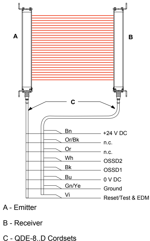
Figure 6. Individual cordsets
