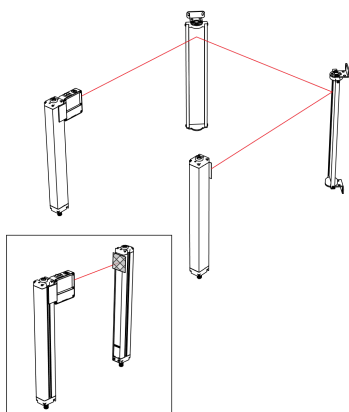
Figure 25. Optical alignment using the LAT-1
