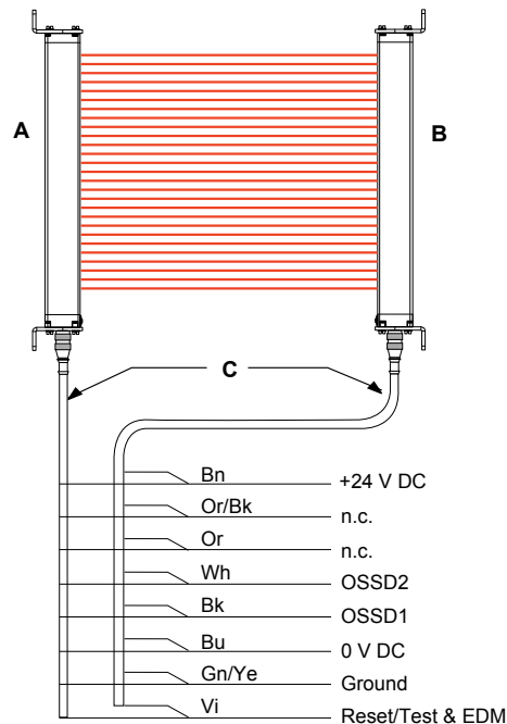
Figure 21. Individual cordsets
