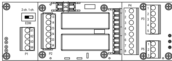
Wiring—model EZAC-R9-QE8
