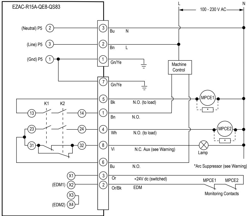
Wiring—model EZAC-R15A-QE8-QS83
