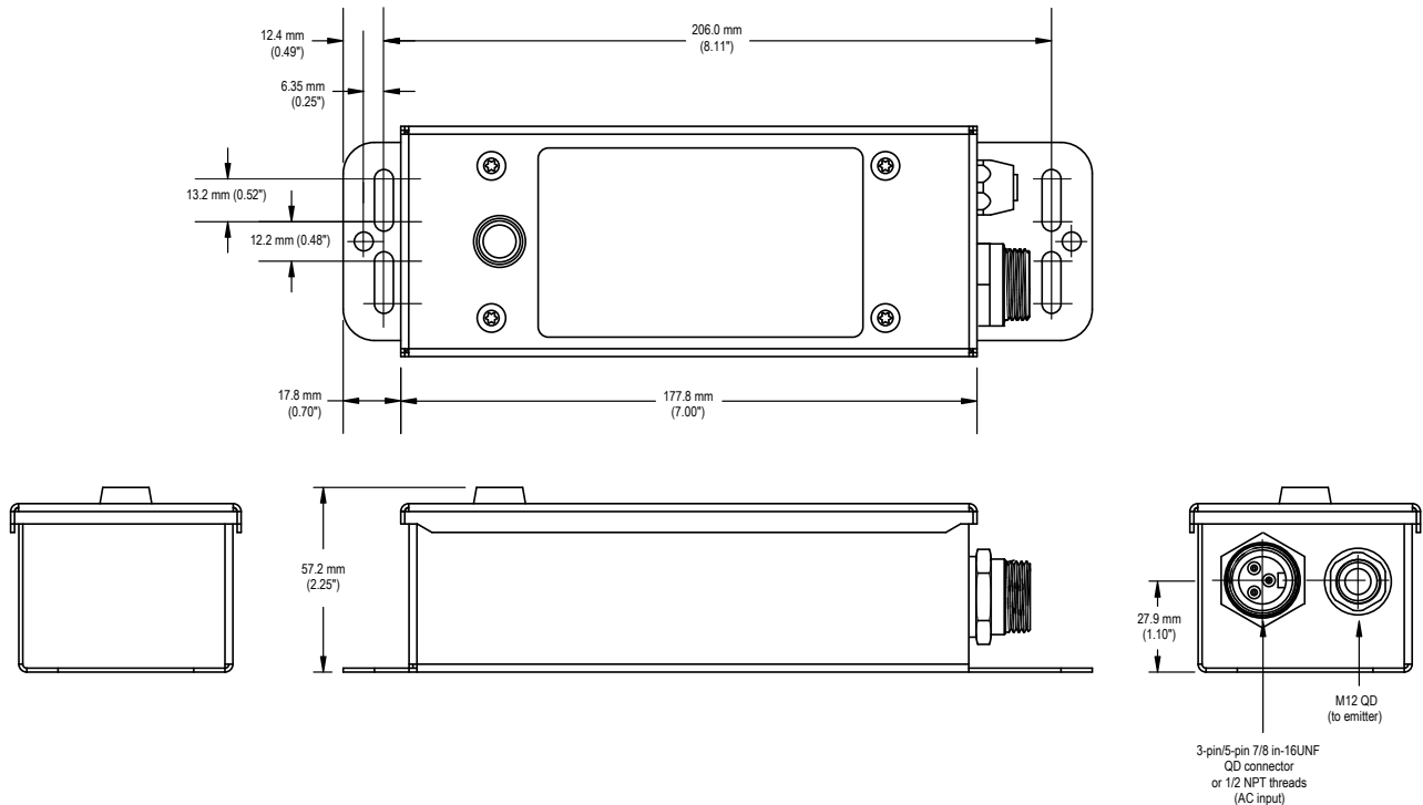
Model EZAC-E.. EZ-SCREEN AC Interface Box
