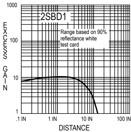
Figure 9. Excess Gain
