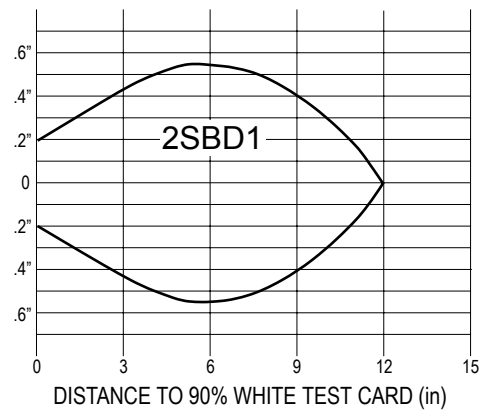
Figure 10. Beam Pattern
