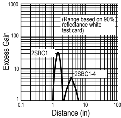
Figure 7. Excess Gain
