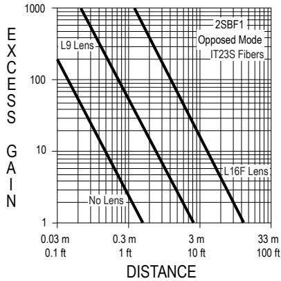
Figure 13. Excess Gain - Opposed
