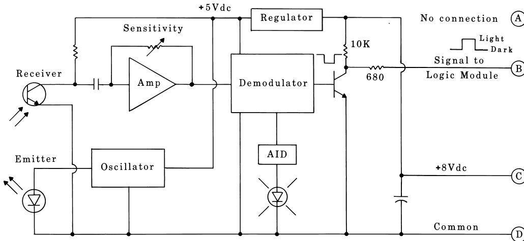
Figure 2. Functional Schematic
