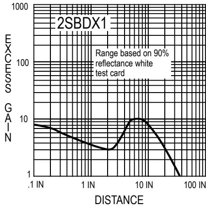
Figure 11. Excess Gain
