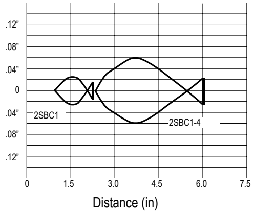
Figure 8. Beam Pattern
