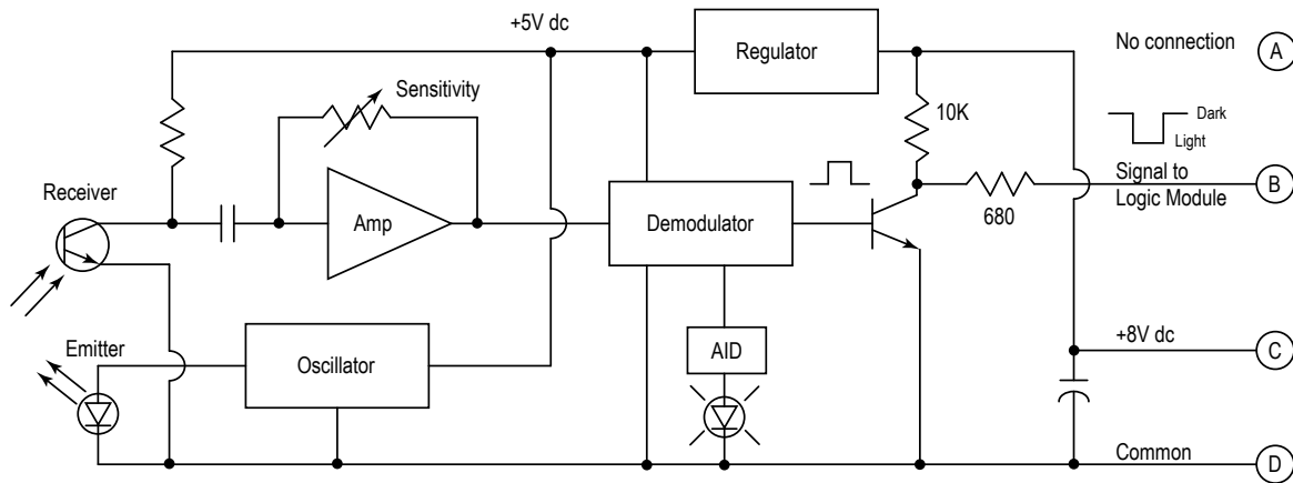
Figure 1. Functional Schematic
