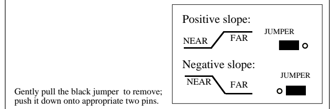
Figure G: ULTRA-BEAM Slope Select Jumper Setting
