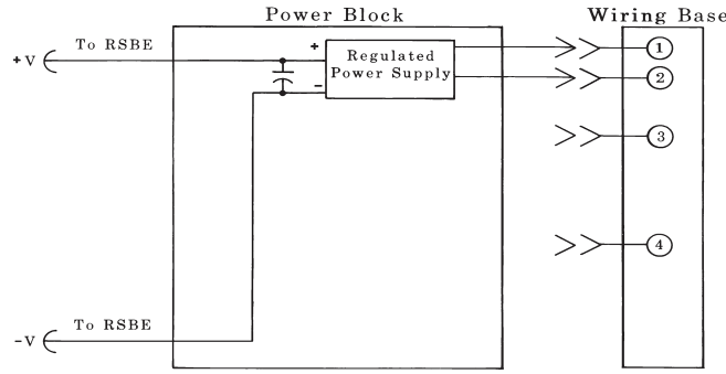
Figure 2. Functional Schematic
