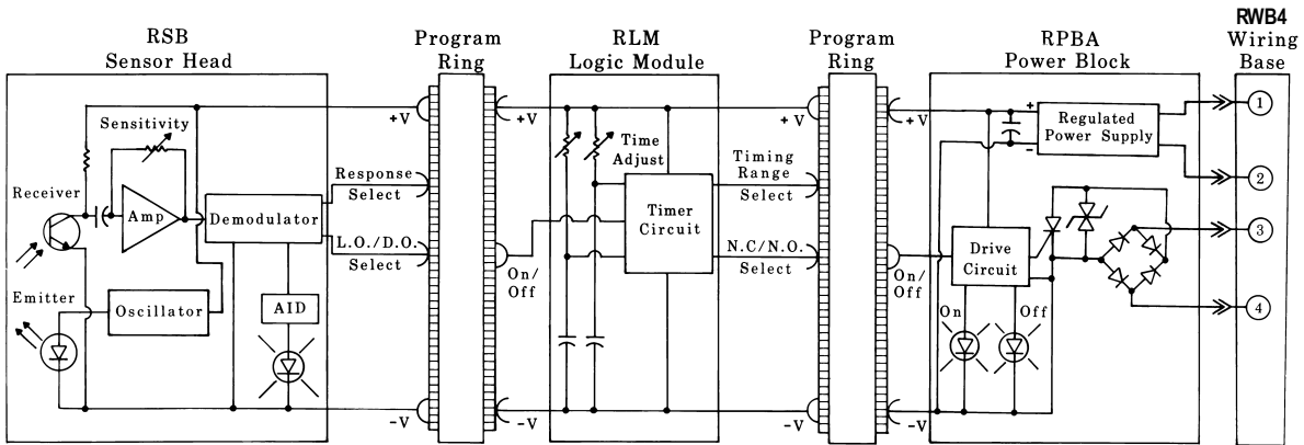
Figure 3. Composite Functional Schematic
