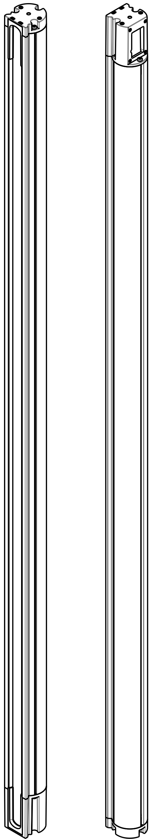
ISOMETRIC VIEWS SCALE 2:5
