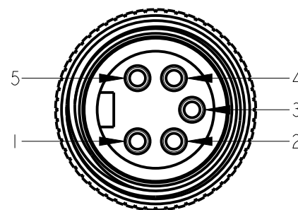
MALE PINOUT
