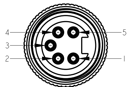
FEMALE PINOUT
