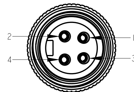
MALE PINOUT
